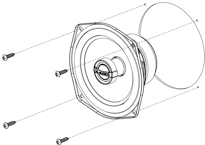
DIAGRAM A: 4-hole Speaker Installation
