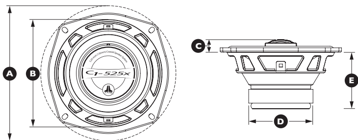
Coaxial Physical Dimensions
