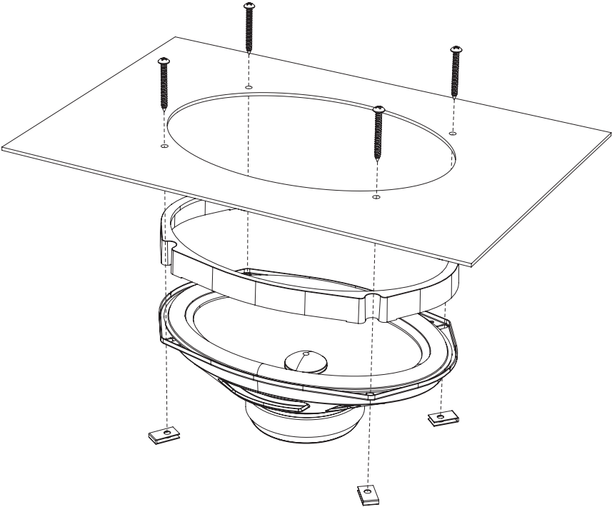
DIAGRAM F: Speaker Installation with Spacer Ring
