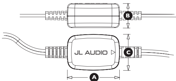
Crossover Network Physical Dimensions
