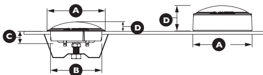
Tweeter Fixture Physical Dimensions
