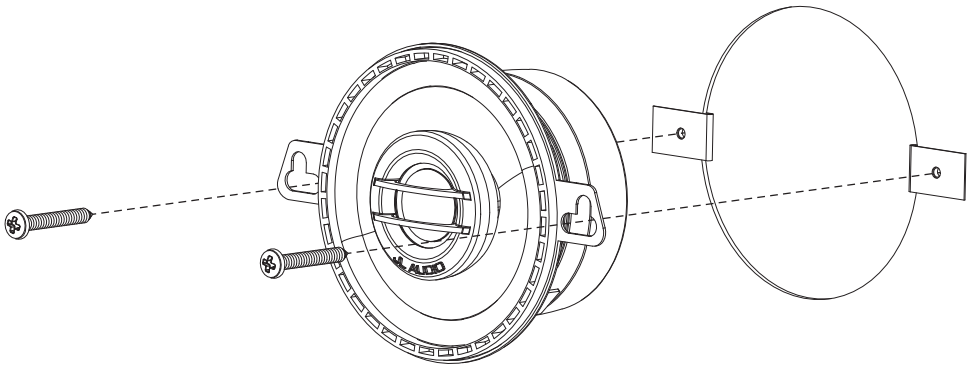
Diagram A: Factory & Custom Location Woofer Installation
