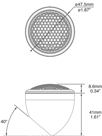
With housing for angle mount
