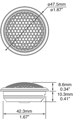
With housing for flush mount
